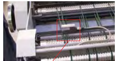
UP3092 4 Pin Sensor (230-434-0100)
