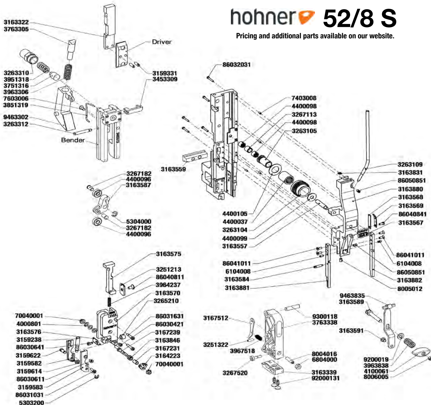
4400037 One Way Bearing
