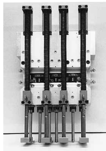
LAWSON MULTI-SPINDLE DRILL HEADS 2-3-4-5-6-7-8
