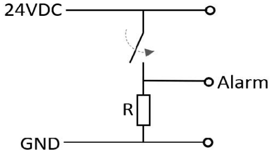
Simplified Diagram of NPN output
