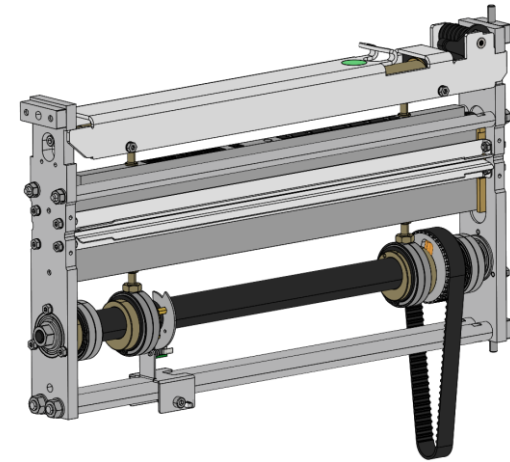
Creaser – Static Creasing Unit
