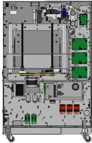
Feeder – Rear Side
