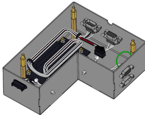
Feeder – Options
