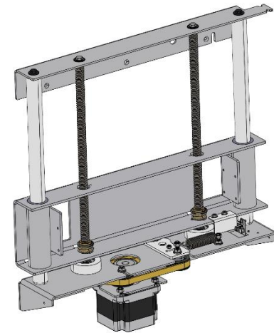
Feeder – Lift Mechanism
