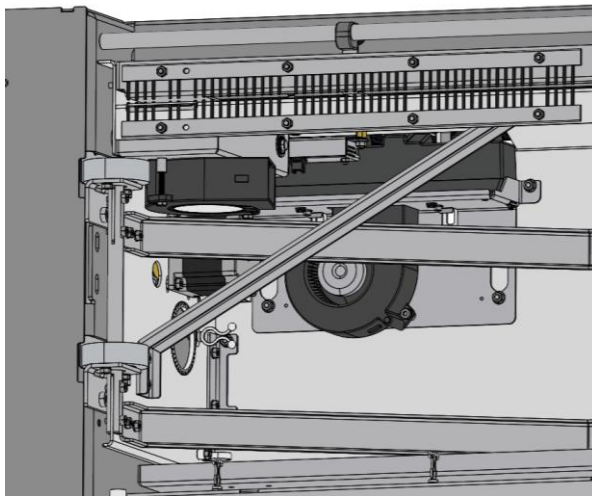
Feeder – Exit Side
