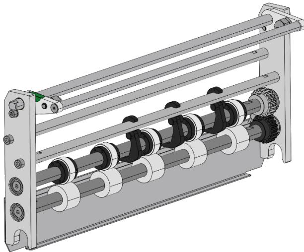
Creaser – Rotary Tool Carrier
