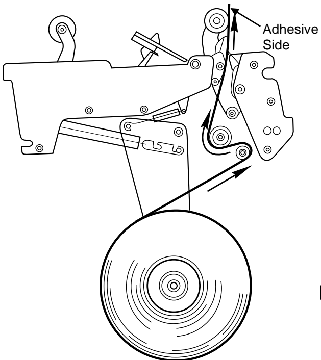
Bottom Cartridge
